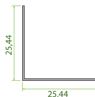
CANTONEIRA L 1"
