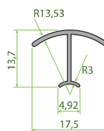
CANTONEIRA REDONDA
